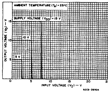
Fig. 1 - Typical voltage transfer characteristics.
