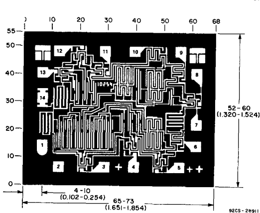
CD4000B
