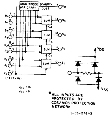
Fig. 1 — CD4008B logic diagram.
