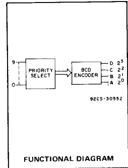
FUNCTIONAL DIAGRAM
