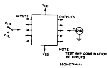
Fig. 14 - Input voltage test circuits.
