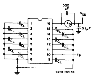
Fig. 12 - Dynamic power dissipation test circuit for CD4020B.
