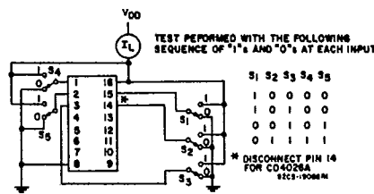
Fig. 15 - Quiescent device current test circuit.
