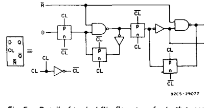
Fig. 5 - Detail of typical flip-flop stage for both types.
