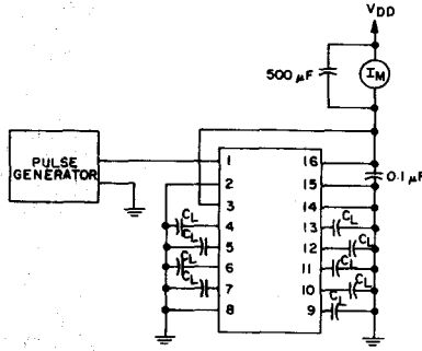
Fig. 14 - Dynamic power dissipation test circuit for CD4033B.
