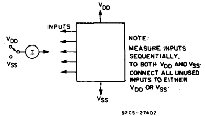
Fig. 17 - Input current.
