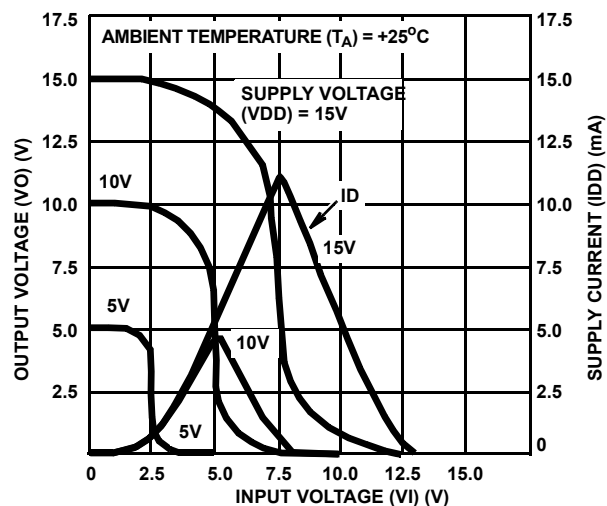
FIGURE 4. TYPICAL CURRENT AND VOLTAGE TRANSFER CHARACTERISTICS
