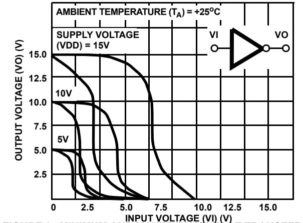
FIGURE 2. MINIMUM AND MAXIMUM VOLTAGE TRANSFER CHARACTERISTICS
