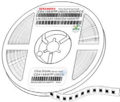
Plastic reel front side
