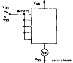
Fig.10 – Quiescent device current test circuit.
