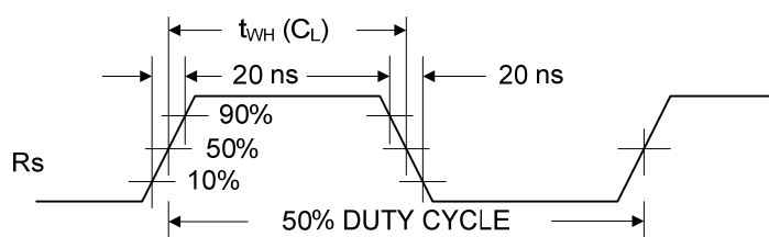
Switching Time Test Circuit and Waveforms
