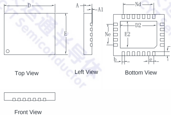
WQFN24
