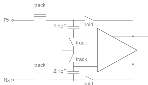
Figure 2. Input Configuration
