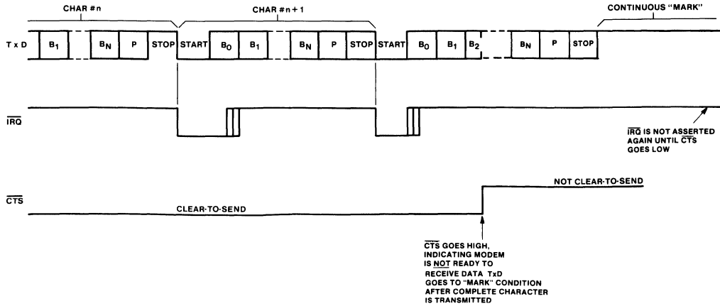
Fig. 10 - Effect of \overline{\text{CTS}} on transmitter.
