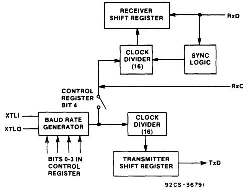
Fig. 6 - Transmitter receiver clock circuits.
