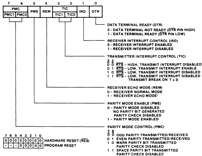
Fig. 5 - CDP65C51A command register.
