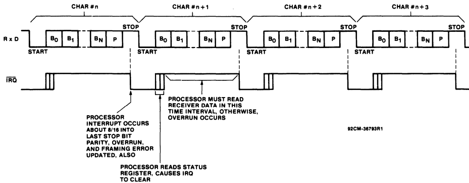
Fig. 8 - Continuous data receive.
