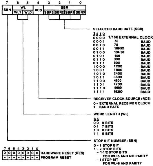
Fig. 4 - CDP65C51A control register.
