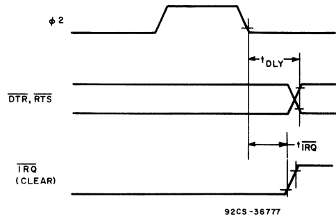
Fig. 24 - Interrupt-and output-timing waveforms.
