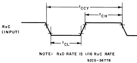
Fig. 25 - Receive external clock timing waveforms.
