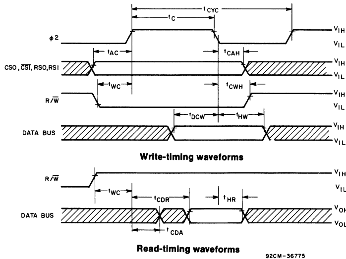
Fig. 22 - Timing waveforms.
