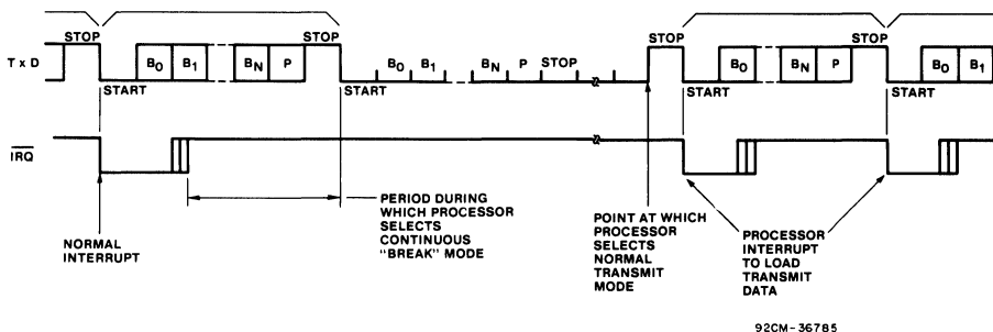
Fig. 18 - Transmit continuous "BREAK".
