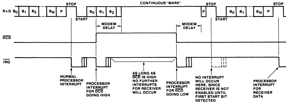
Fig. 16 - Effect of \overline{DCD} on receiver.
