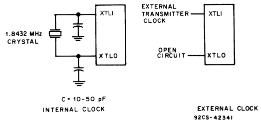
Fig. 26 - Transmitter clock generation.
