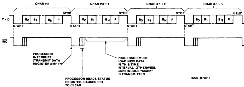
Fig. 7 - Continuous data transmit.
