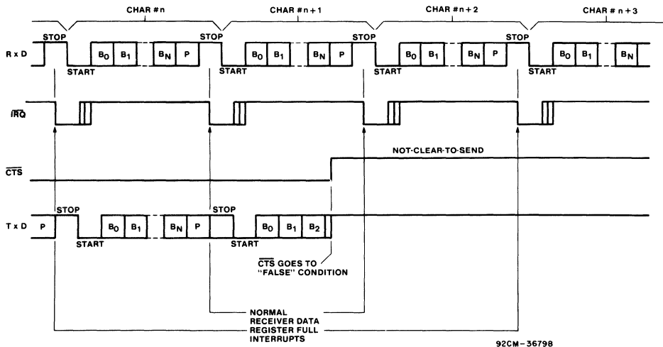
Fig. 13 - Effect of CTS on echo mode.
