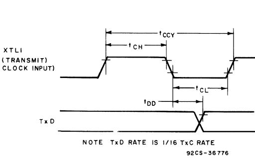
Fig. 23 - Transmit-timing waveforms with external clock.
