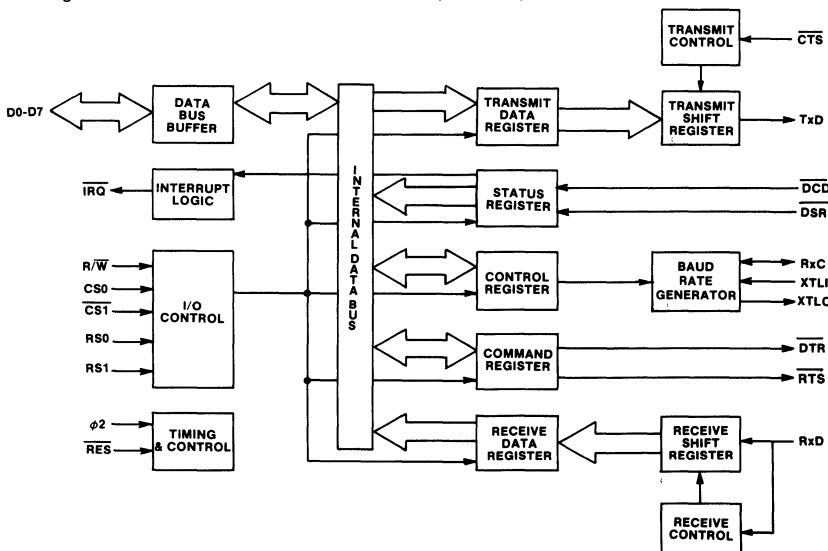
Fig. 2 - Internal organization.
