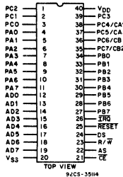
40-Lead Packages
