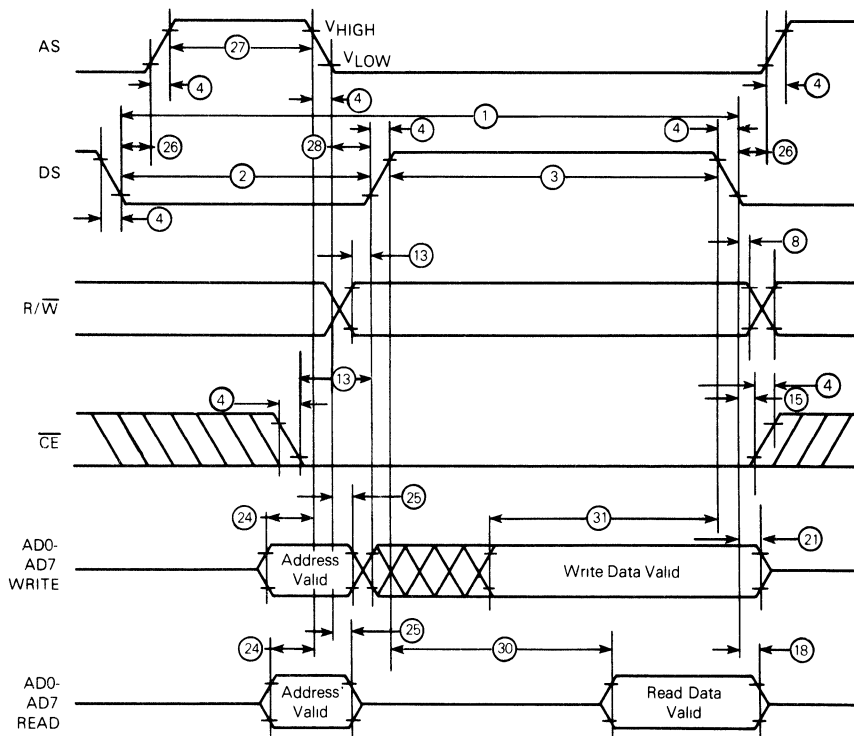
Fig. 3 - Bus timing diagram.
