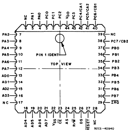
44-Lead Plastic Chip-Carrier Package
