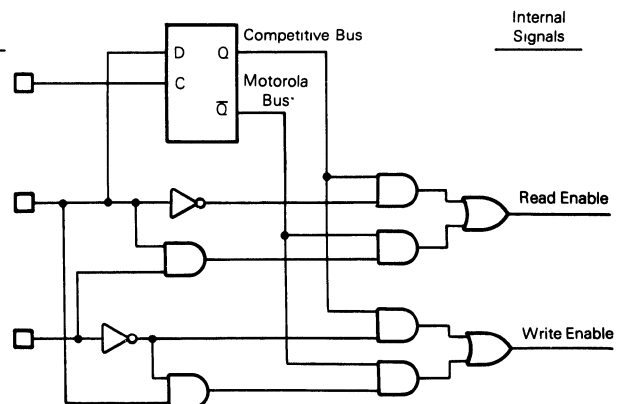
Fig. 7 - Functional diagram of MOTEL circuit.
