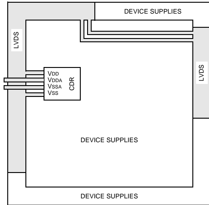
Figure 7. Power Supply Connections
