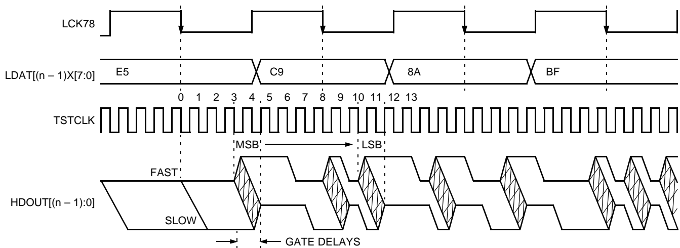
Figure 5. 622.08 Mbits/s Transmit (PLL Bypass Mode) Timing
