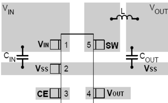
Figure2(a) CE8509A18M Suggested Layout
