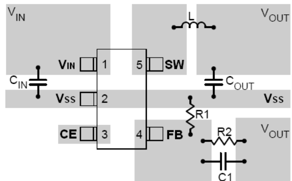
Figure2(b) CE8509AM Suggested Layout
