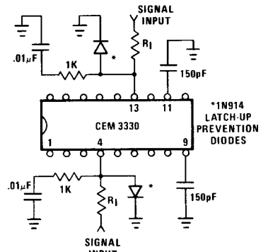
FIGURE 5: GAIN CELL COMPENSATION FOR LARGER BANDWIDTH
