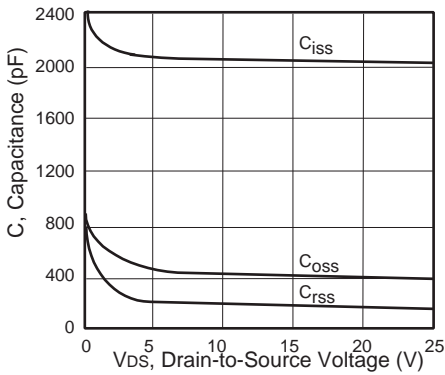
Figure 3. Capacitance
