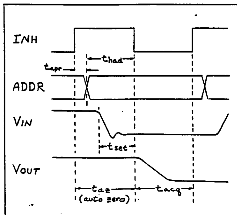
FIG. 1: CEM5530 TIMING
