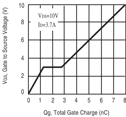
Figure 9. Gate Charge
