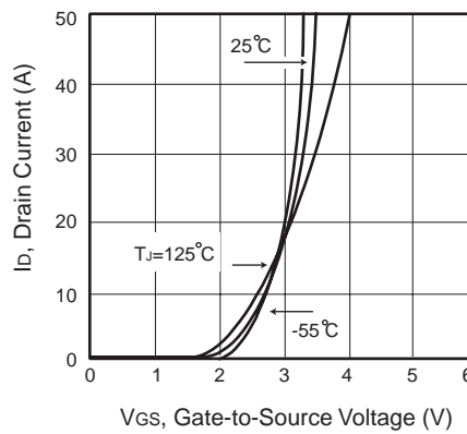
Figure 2. Transfer Characteristics
