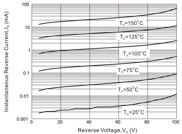
Fig. 2 - Reverse Characteristics (per diode)
