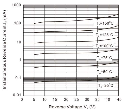
Fig. 3 - Reverse Characteristics
