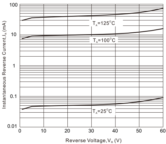
Fig. 2 - Reverse Characteristics
