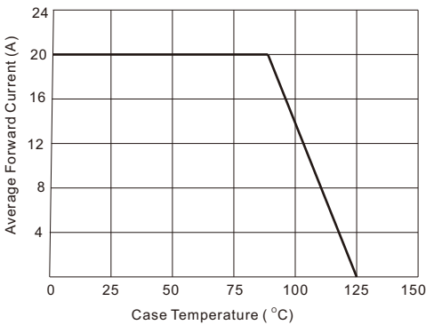
Fig. 4 - Forward Current Derating Curve (Per Diode)
