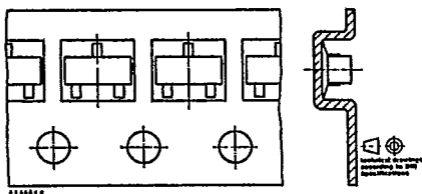
Fig. 7.6 Reverse taped SOT 23
