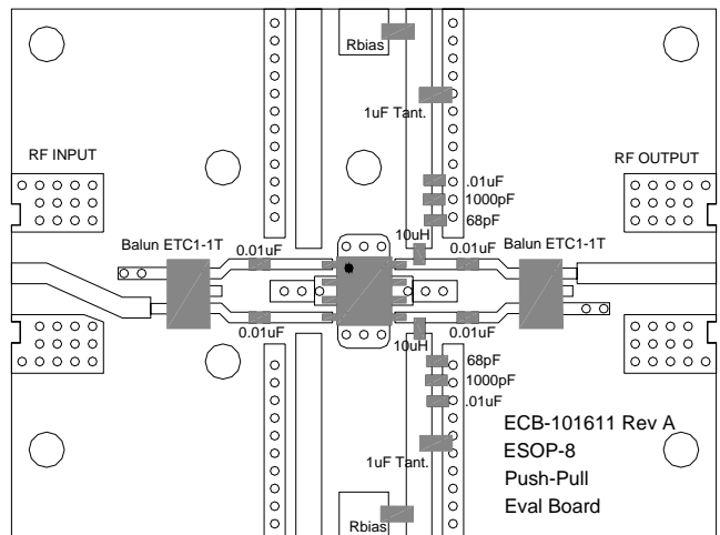
5-100 MHz Evaluation Board Layout
