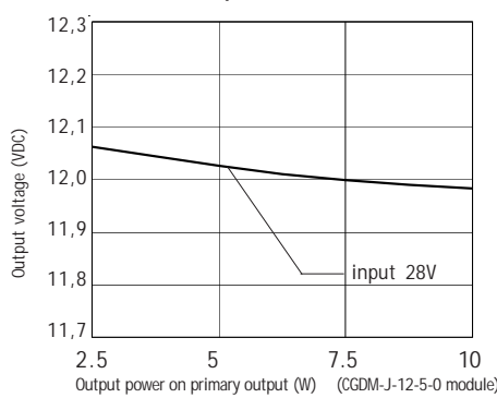
Figure 11 : Typical load regulation characteristics on secondary output 12Vdc at nominal input
