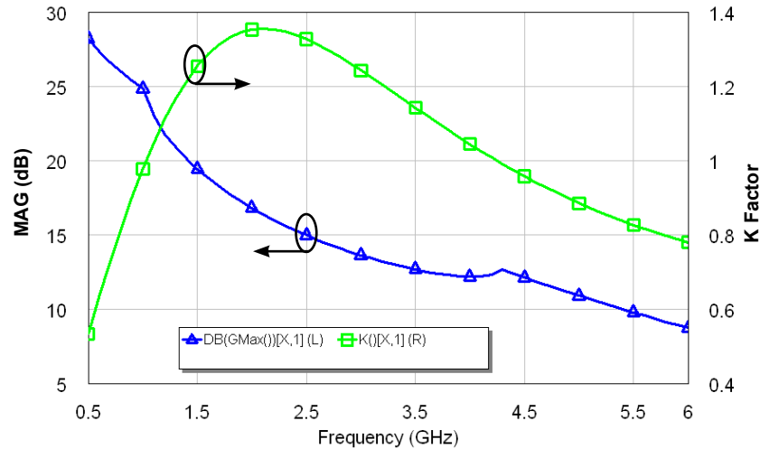
Simulated Maximum Available Gain and K Factor of the CGH40120F V_{DD} = 28\text{ V}, I_{DQ} = 1.0\text{ A}
