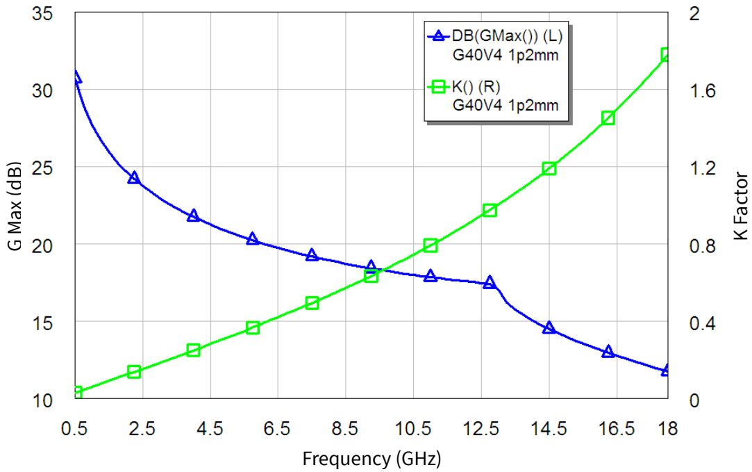
CGHV1J006D - Stability with Gmax and K Factor
