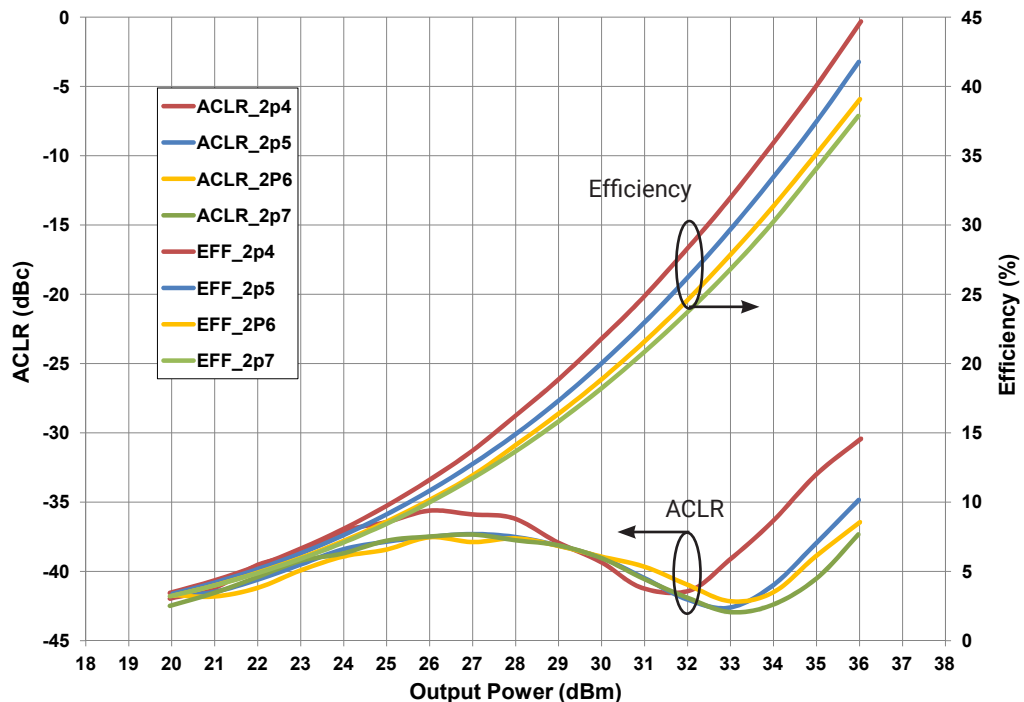
Figure 2. - Typical Drain Efficiency and ACLR vs. Output Power V_{DD} = 50\text{ V}, I_{DQ} = 60\text{ mA}, 1\text{ Carrier WCDMA}, PAR = 7.5\text{ dB}
