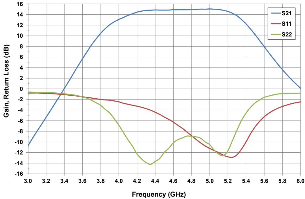
Figure 1. - Small Signal S-parameters CGHV50200F in Test Fixture V_{DD} = 40\text{ V}, I_{DQ} = 1\text{ A}, T_{case} = 25^\circ\text{C}
