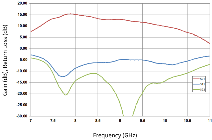
Figure 1. Small Signal Gain and Return Loss vs Frequency of CGHV96100F2 measured in CGHV96100F2-AMP V_{DS} = 40\text{ V} , I_{DQ} = 1000\text{ mA}
