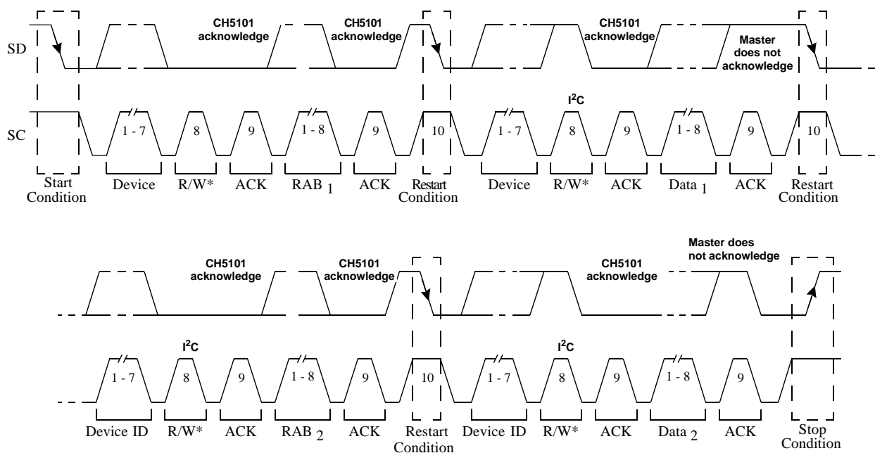
Figure 10: Alternating Read Cycle
