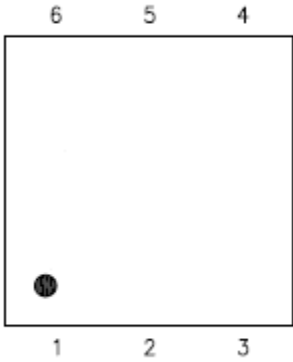
Figure 3: DFN-6 Pin Out
