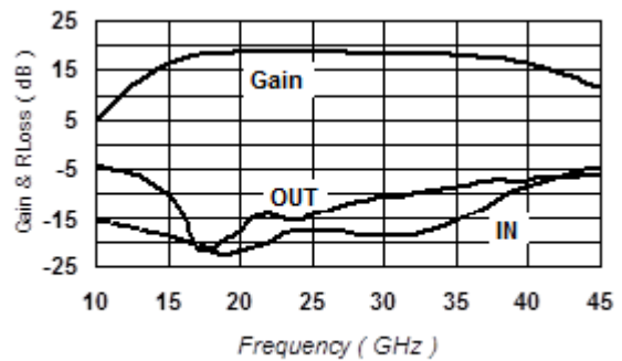
Typical on wafer measurement
