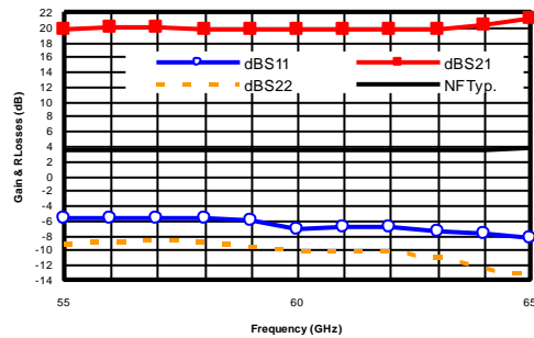
Typical on wafer measurement
