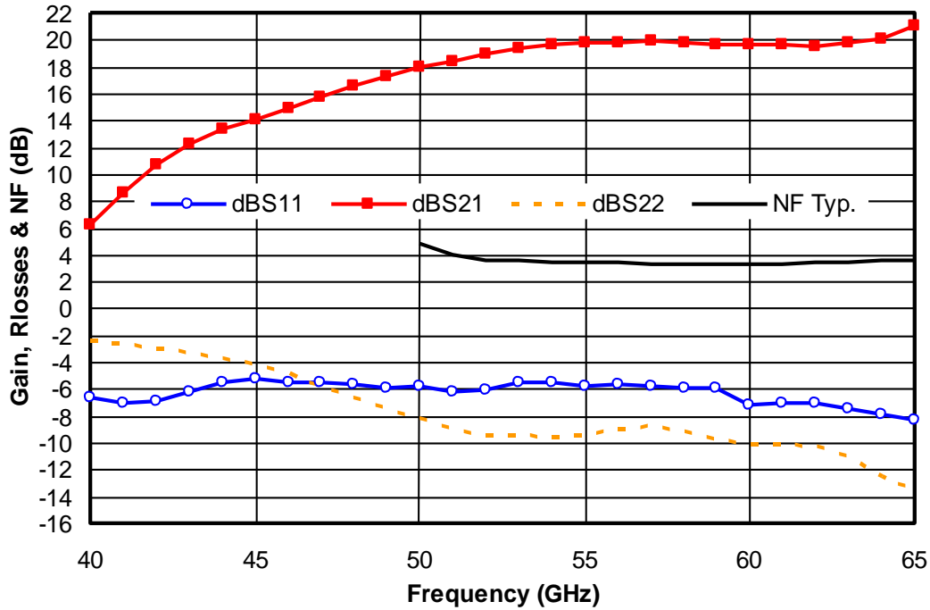
Typical Gain, Return Losses and Noise figure
