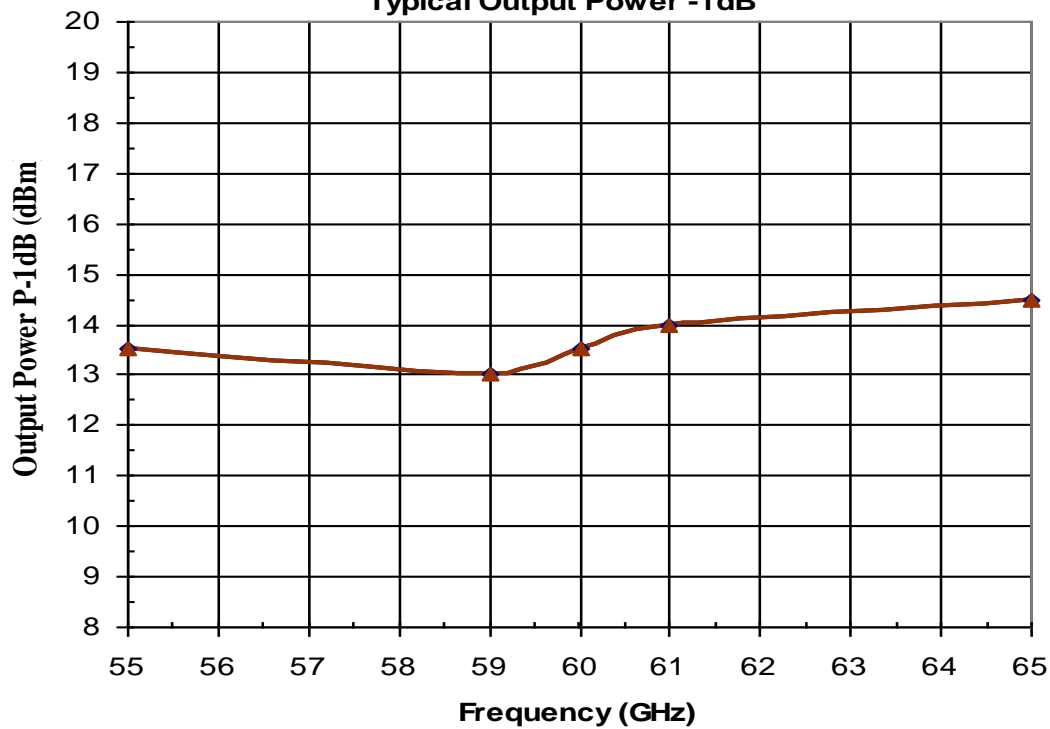
Typical Output Power -1dB
