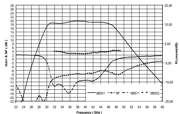
On wafer typical measurement
