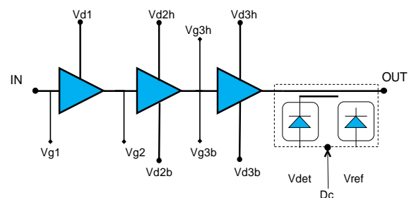
Functional diagram
