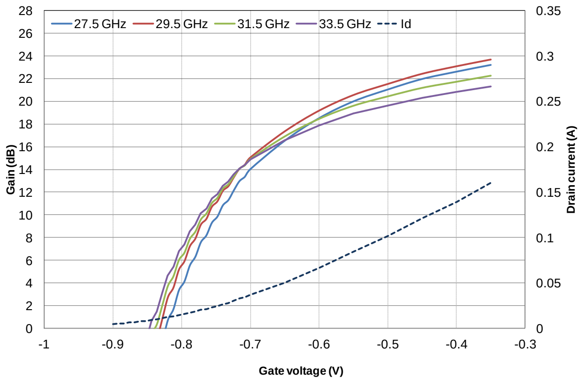
Linear gain & Current versus Gate Voltage
