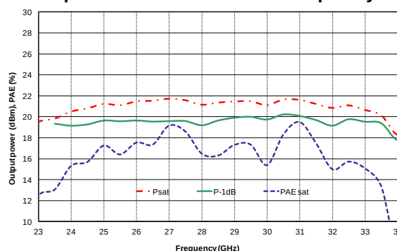
Output Power & PAE versus Frequency
