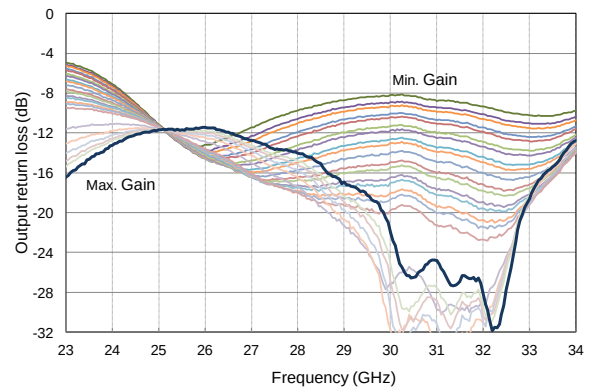
Output return loss versus gain ctrl
