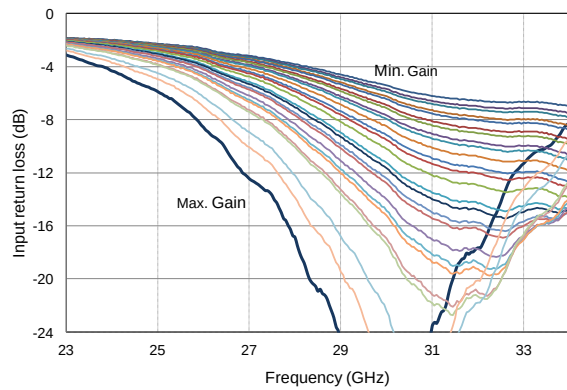
Input return loss versus gain ctrl
