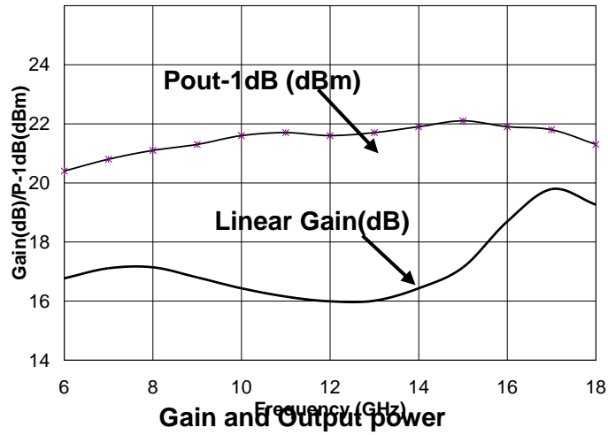
Linear Gain & Output Power for 1 dB compression Versus frequency Test fixture measurement
