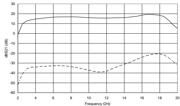
Typical on wafer Measurements Gain versus switch states
