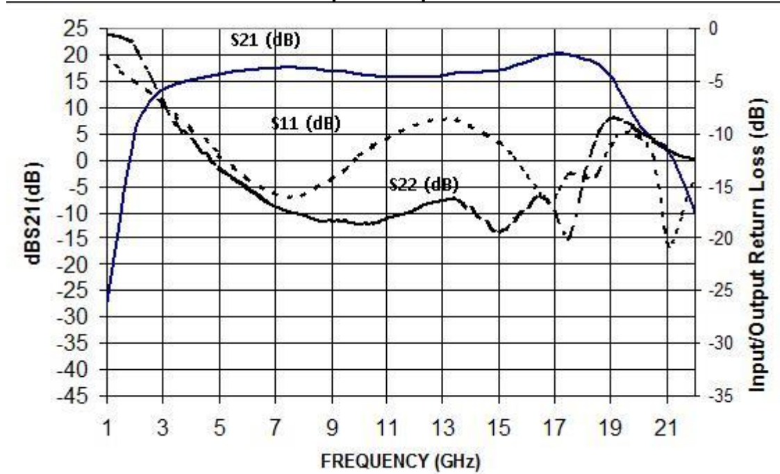
Configuration Gain ( Pad E2=-5V/ Pad F=0V) Gain/ input & output Return Loss
