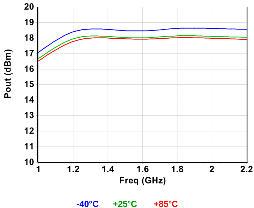
Output power @ Sat versus Frequency
