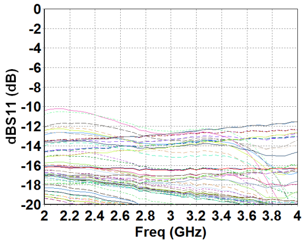
Input Return Loss versus Frequency (all states)
