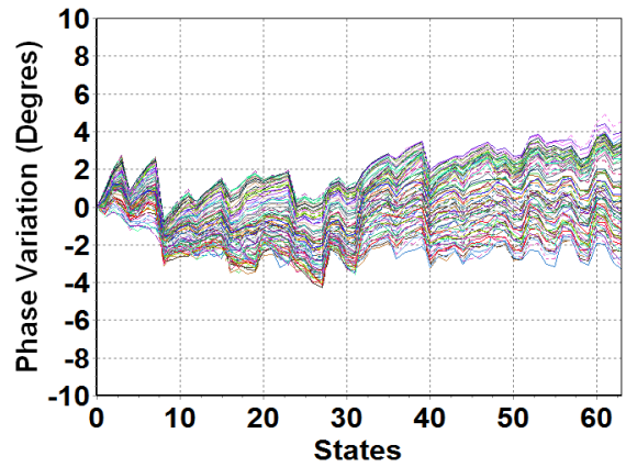
Phase Variation versus States (Frequency 2-4GHz)
