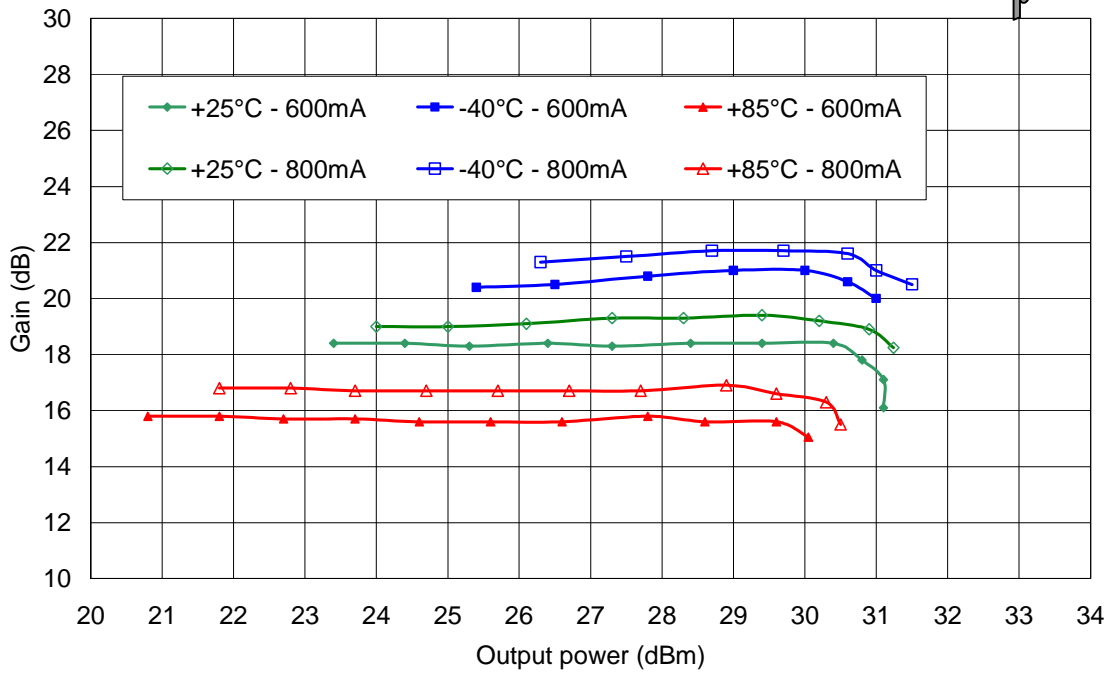
Output power versus temperature & Drain current @ 25.5GHz
