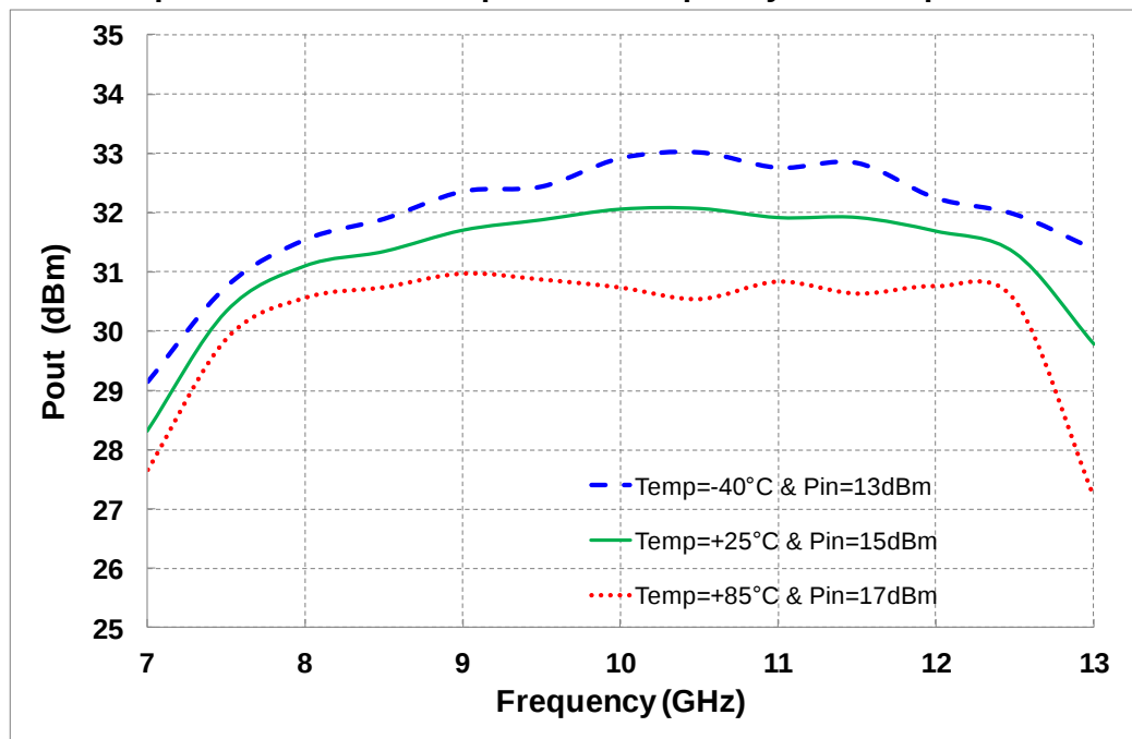
Output Power at 3dBcomp versus Frequency and Temperature
