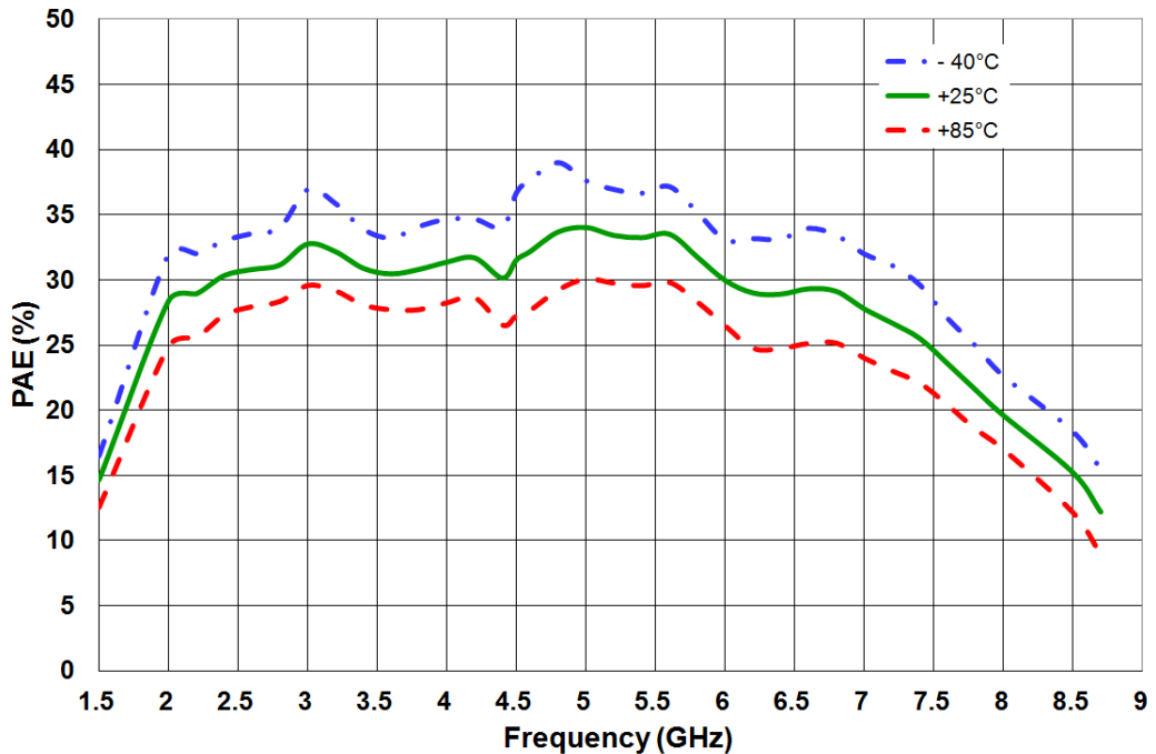
Power added efficiency versus frequency for input power=23dBm at -40°C / 25°C / 85°C
