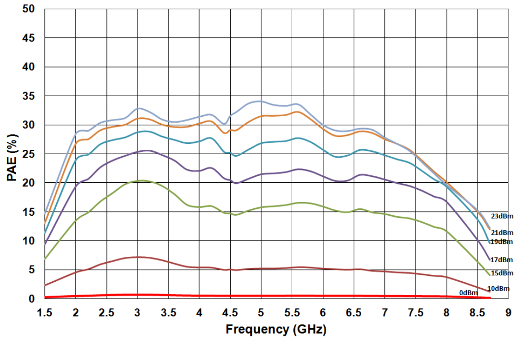
Power added efficiency versus frequency at 25°C for input power=0/10/15/17/19/21/23dBm
