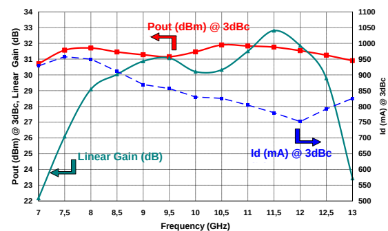
Pout & Id @ 3dB gain compression and Linear Gain (Pulse 25μs 10% Tamb. 20°C)
