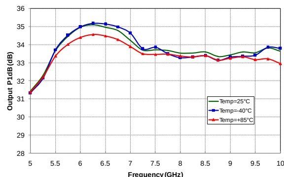
Output power at 1dB comp.
