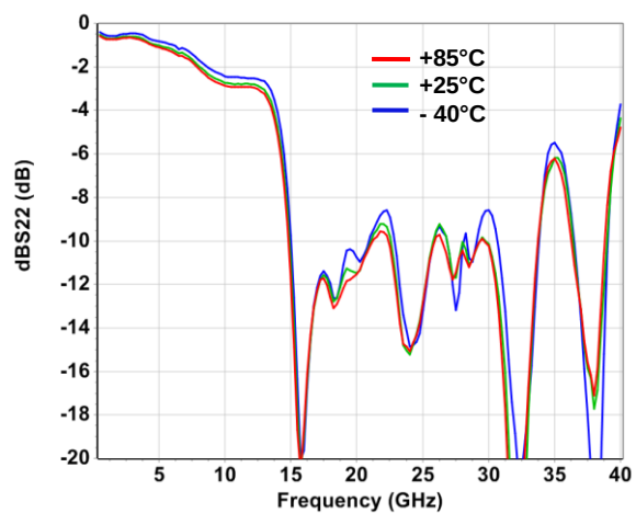
Output Return Loss versus Frequency in Temperature
