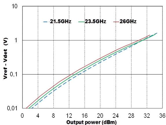
Power Detector versus Pout and Frequency
