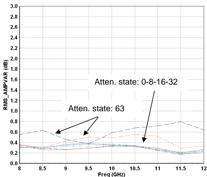
Amplitude variation RMS Tuning attenuator state 1 Fine attenuator states 0-8-16-32
