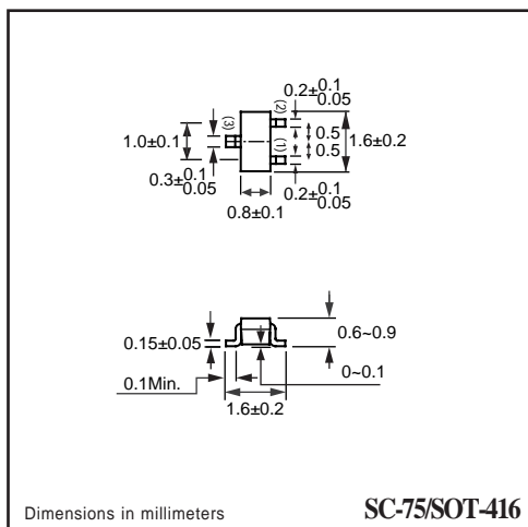
SC-75/SOT-416
